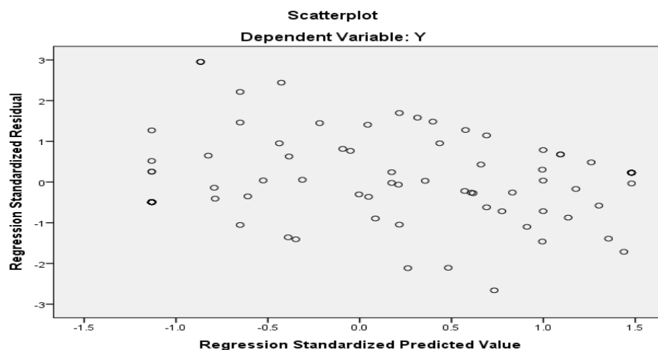
Gambar 2 Scatter Plot Uji Heteroskedastisitas
