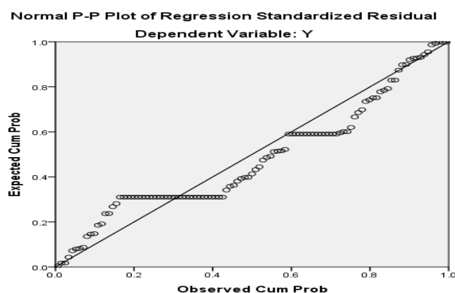
Gambar 1. P. Plot Normalitas Data
